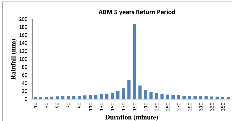
Fig. 3. Hietograph with the ABM Method for a 5 Year Return Period
