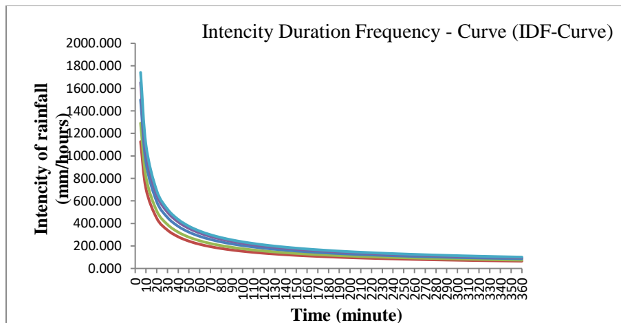
Fig. 2. IDF (Intensity Duration Frequency) Curve
